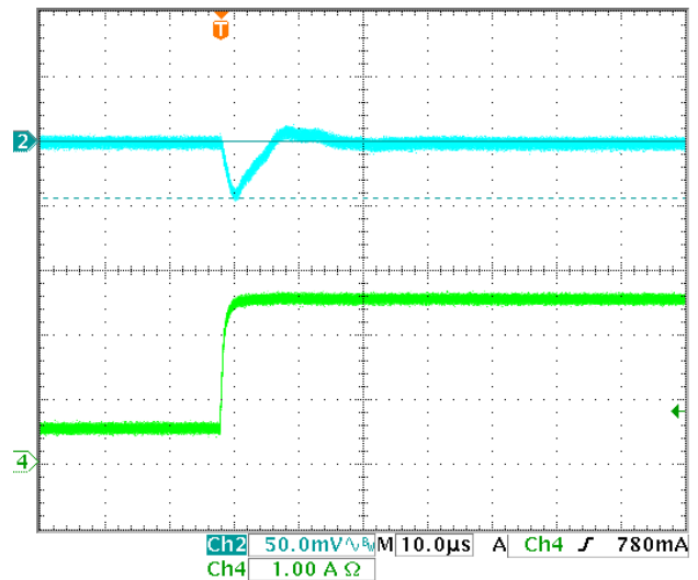
Figure 13 · L = 0.68\mu H , C_{OUT}=44\mu F , Rising Edge
