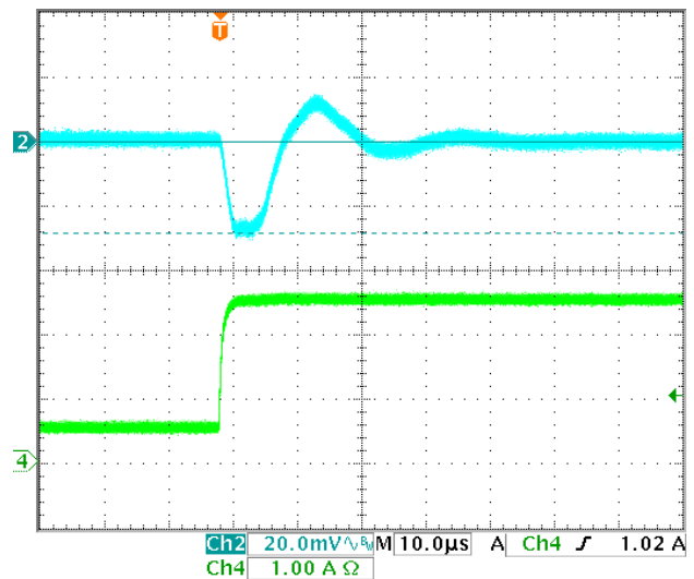
Figure 15 · L = 0.68\mu H , C_{OUT}=154\mu F Rising Edge
